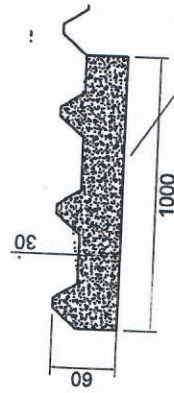
ROOF PANEL
